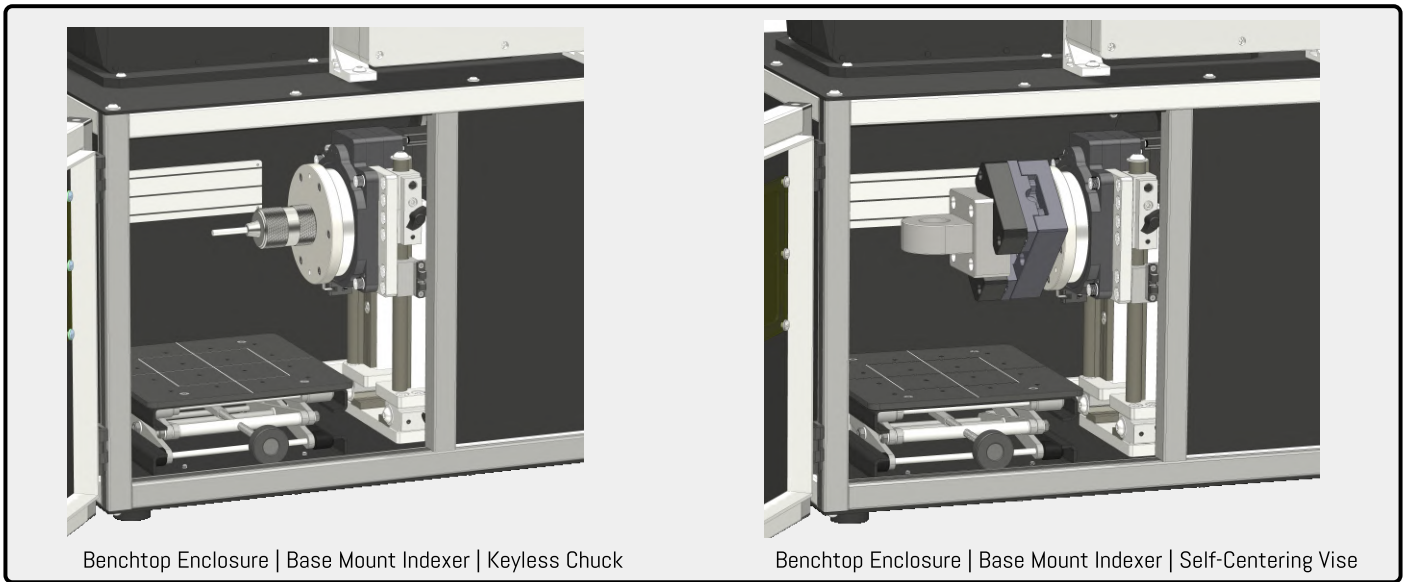
Benchtop Enclosure | Panel Mount Indexer | 3-Jaw Chuck
