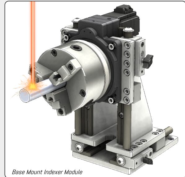
Base Mount Indexer Module
