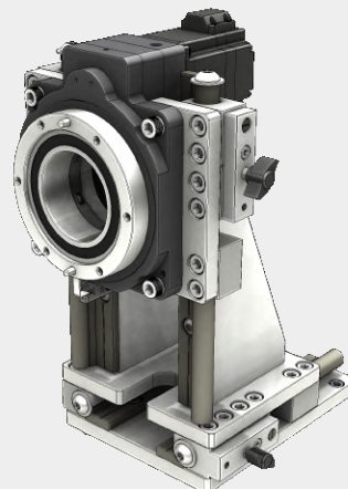
Mounts fully inside laser enclosure. Horizontal & vertical position adjustment.
