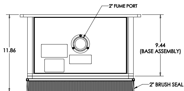
Wide Marking Area Shroud
