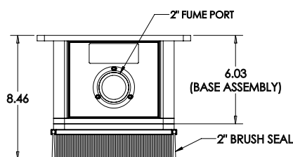
Standard Marking Area Shroud
