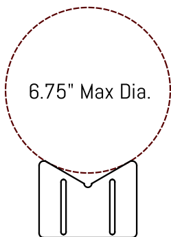
120 Degree V-Notch Bank Plate
