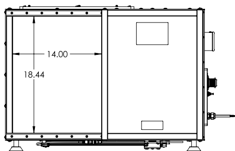
DOORS OPEN
