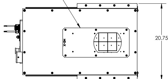
LASER MARKER MOUNT PLATE
