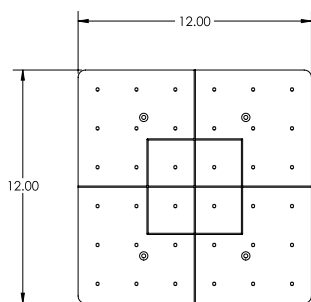
Fixture Plate
